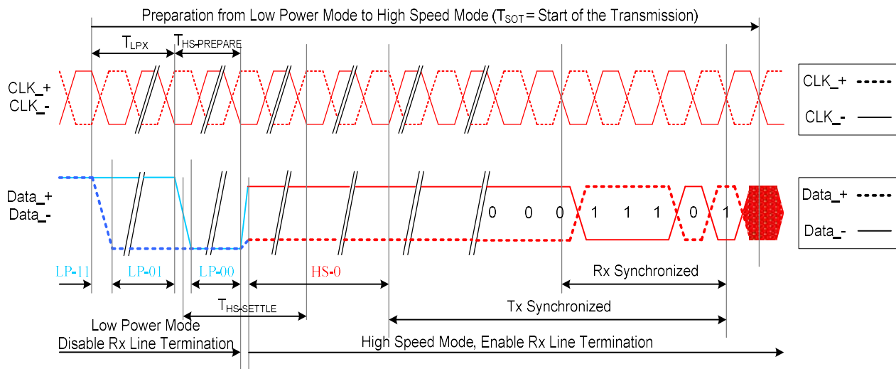
Entering High-Speed Data transmission ( T_{SOT} of HSDT)
