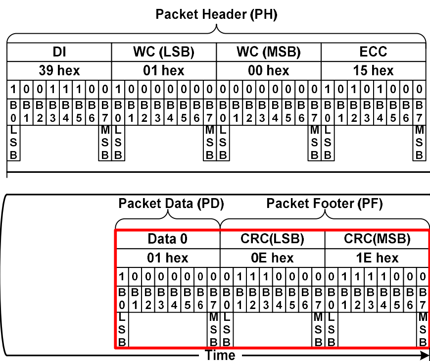
Packet Footer (PF) Example
