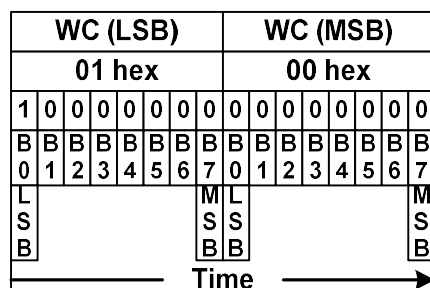
Byte Order of the Multiple Byte on Packets
