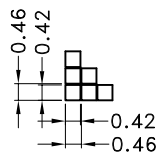
DOT DETAIL SCALE 5:1
