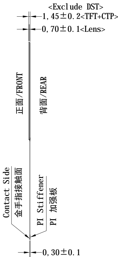
侧视图 Side view
